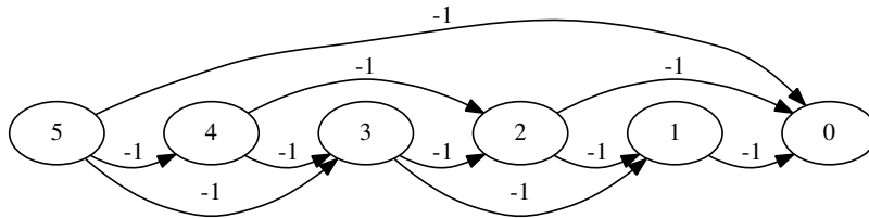
Figure 8.1: The Change-making Problem, formulated as finding the shortest path in a DAG, for K = 5 .
