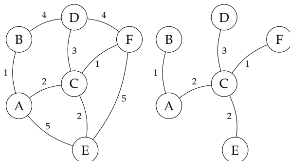
Figure 12.7: A graph with a corresponding minimum spanning tree.
